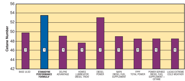
CETANE NUMBER CHANGE
